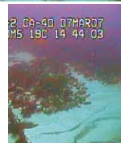
LIVE VIDEO RECORDINGS SHOWING PARTIALLY OVERGROWN CABLE AT HYDROACOUSTIC STATION HA01, CAPE LEEUWIN, AUSTRALIA.
