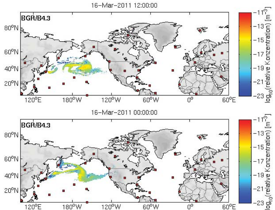
Simulation of dispersion of radioactivity. Courtesy of the German Federal Institute for Geosciences and Natural Resources
